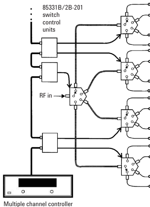
Figure 2. Example of a 1P16T switch configuration constructed from modular components
